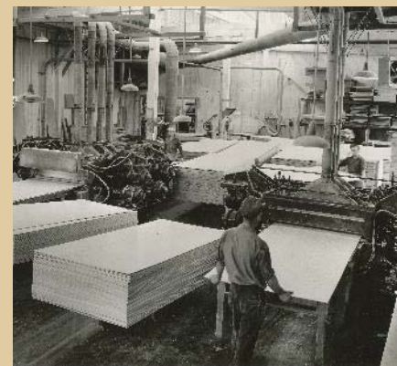
Glued plywood sheets are sanded and trimmed
